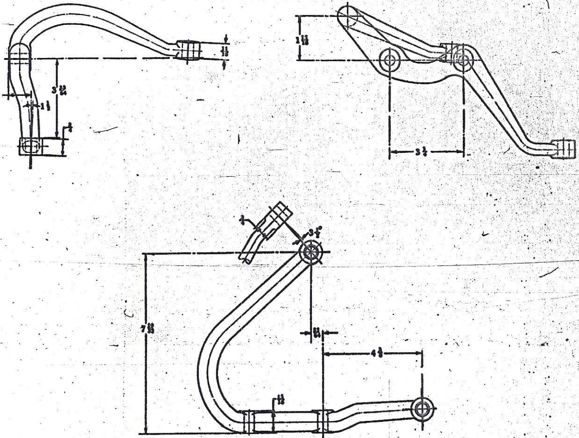
Illustration 31-1-2. Steering Third Arm 1931 Pontiac Six
